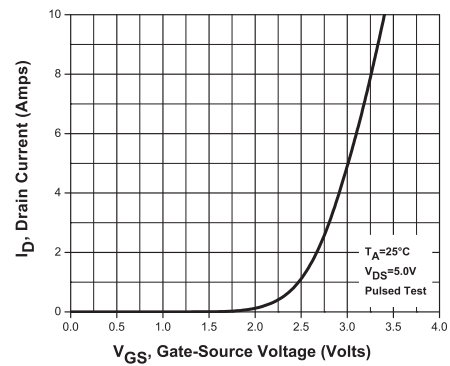
Transfer Characteristics
